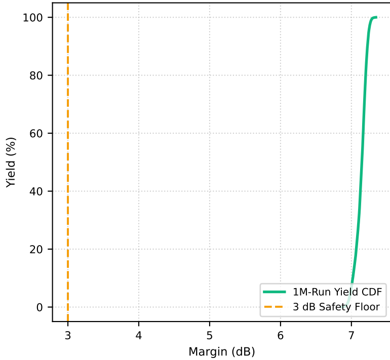
(b) Optical Yield (> 99.99%)
