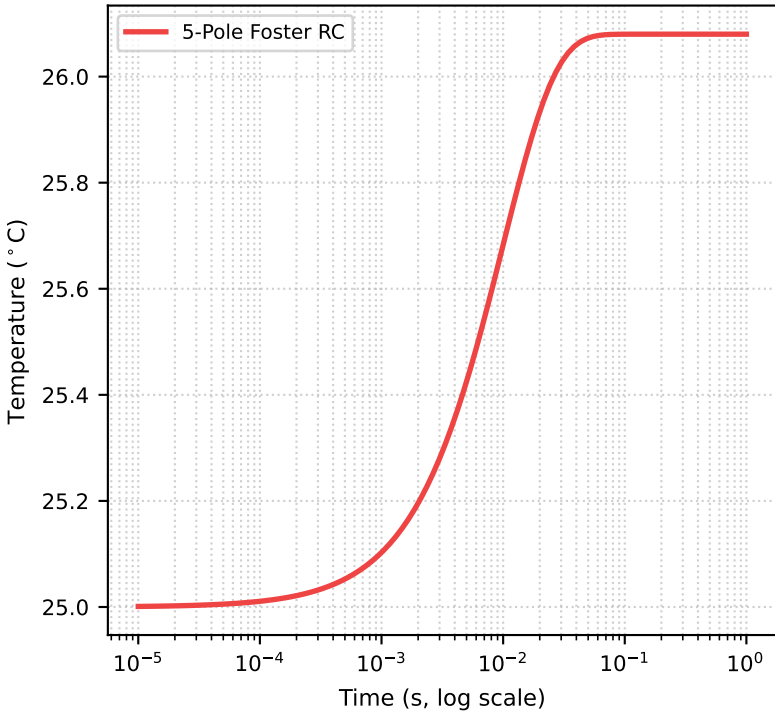
(c) Thermal Step ( T_{\max} = 26.08^{\circ}\text{C} )
