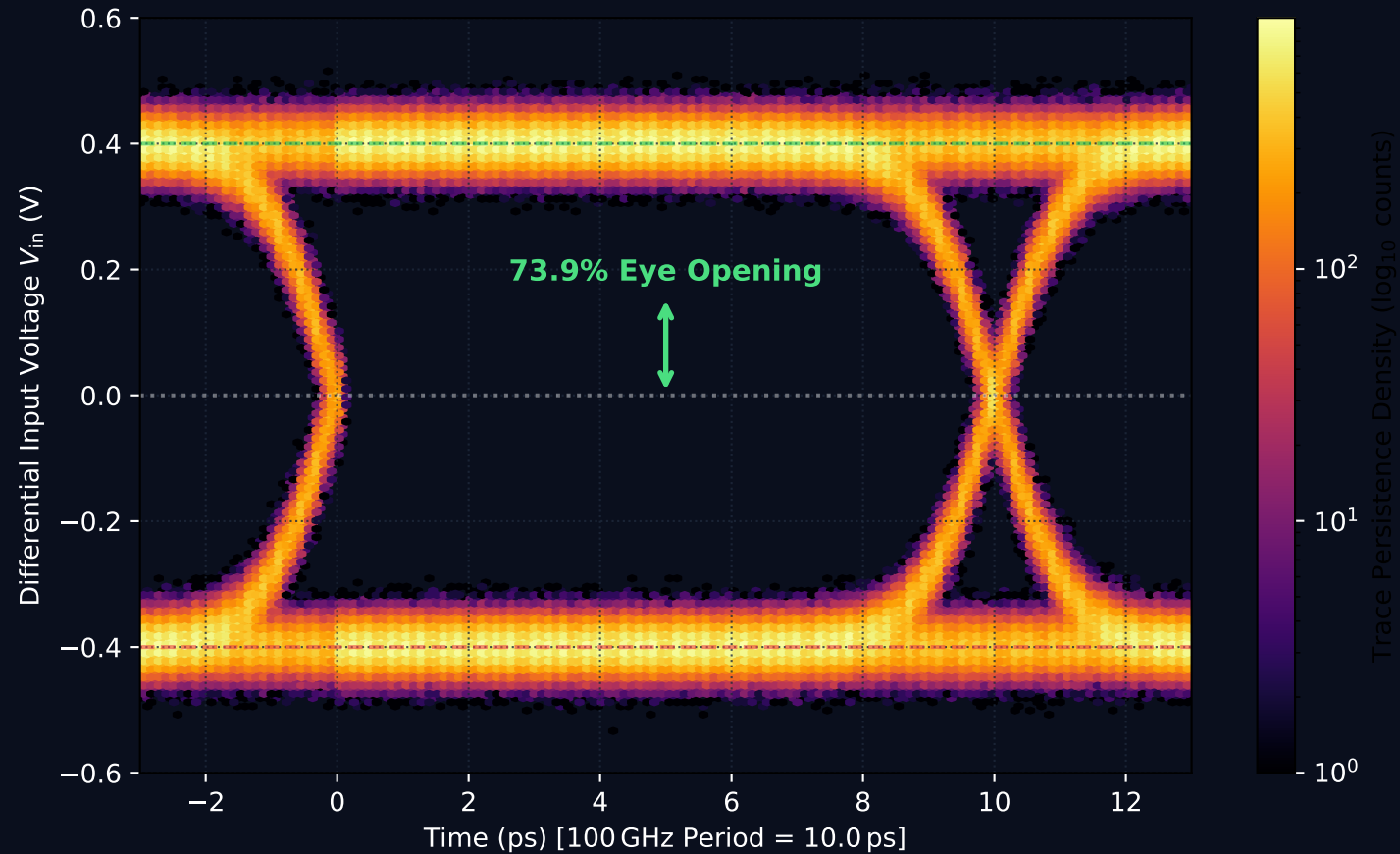
1,000,000-Cycle 100 GHz SPICE: 2D Eye Diagram Persistence Density
