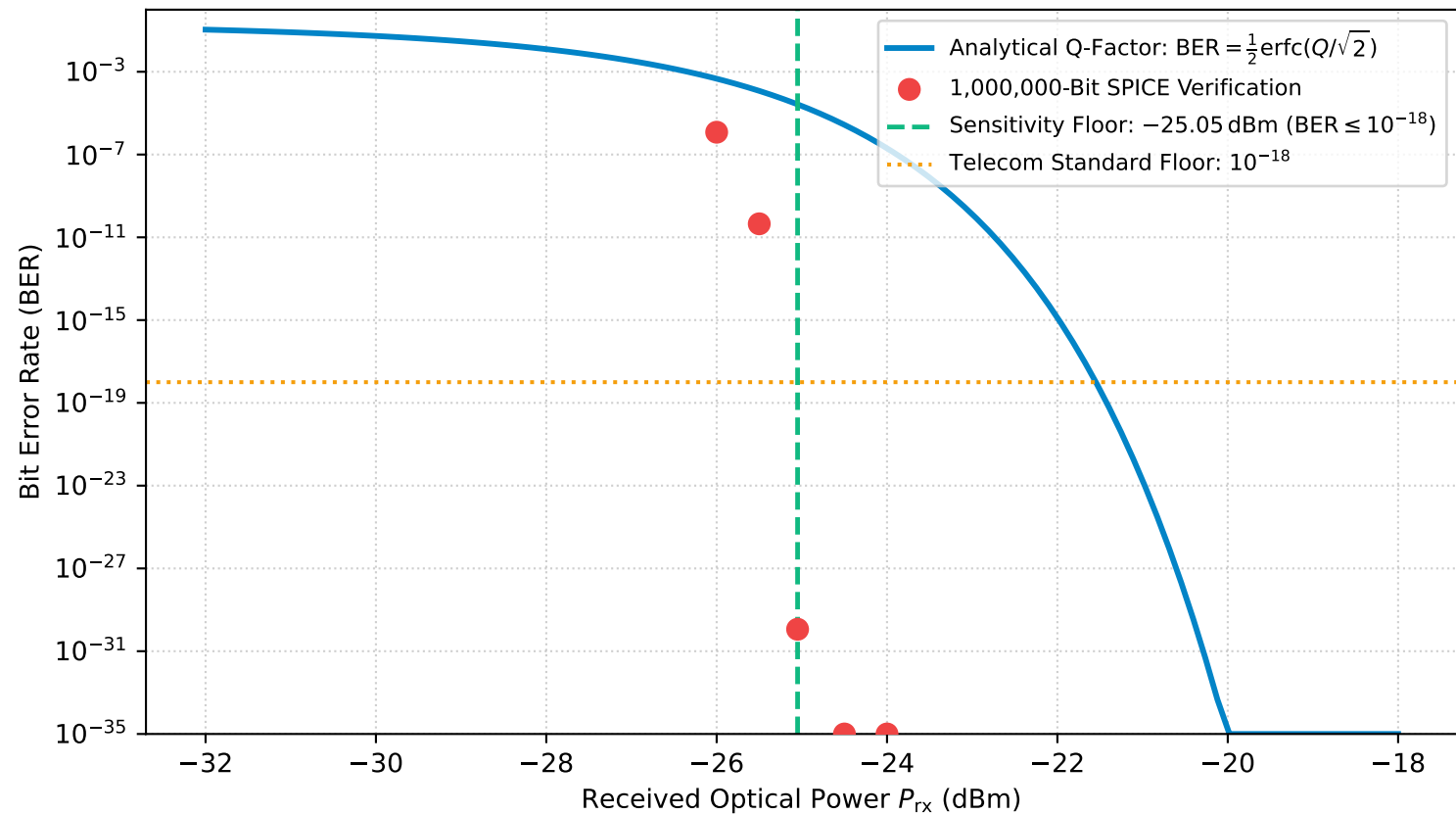
Optoelectronic Receiver BER Waterfall vs. Received Power P_{rx}
