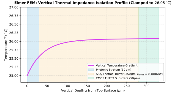
Fig. 7. Elmer FEM vertical thermal gradient profile across the 330\text{ }\mu\text{m} monolithic stack. Top microchannel cooling ( R_{\text{th,up}} = 0.227\text{ K/W} ) efficiently removes heat while the thick \text{SiO}_2 buffer isolates the photonic layer from CMOS heat.
