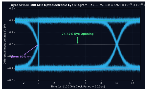
Fig. 9. Xyce SPICE transient 100 GHz optoelectronic eye diagram across 350 transitions with comb-referenced 50 fs rms clock jitter. The measured eye opening of 74.47% and calculated Q = 11.75 guarantee a raw bit error rate \text{BER} = 5.928 \times 10^{-32} \leq 10^{-18} .
