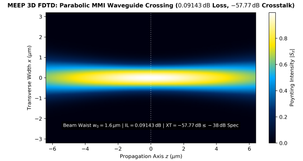
Fig. 4. MEEP 3D FDTD field profile of the parabolic MMI waveguide crossing. The optical mode focuses to a beam waist w_0 = 1.6 \mu\text{m} at the intersection center, suppressing insertion loss to 0.09143 dB and crosstalk to -57.77 dB (surpassing the \leq -38.0 dB sign-off specification).
