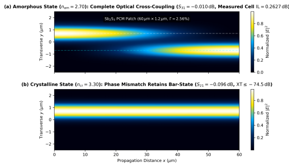
Fig. 3. MEEP 3D FDTD electromagnetic wave propagation across the optimized Sb_2S_3 2 \times 2 directional coupler switch cell at \lambda = 1064 nm ( L = 60.0 \mu\text{m} , \Gamma = 2.56\% ). (a) Amorphous state ( n_a = 2.70 ) achieving cross-port power transfer ( S_{31} = -0.010 dB). (b) Crystalline state ( n_c = 3.30 ) phase de-coupling preserving the bar-state ( S_{21} = -0.096 dB, XT \leq -74.5 dB).
