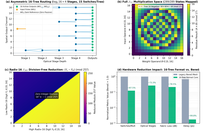
Fig. 5. Architectural formalization of the Asymmetric 16-Tree Fermat Core. (a) 4-stage binary tree routing fabric ( \log_2 16 = 4 ) with 17-channel spatial alphabet ( WG_0 \dots WG_{16} ). (b) Complete \mathbb{Z}_{17} multiplication residue space (289/289 states mapped, 100% state efficiency) and Tree 16 negation symmetry ( 16 \times W \equiv -W \pmod{17} ). (c) Radix-16 \mathbb{Z}_{257} division-free modular reduction: (Y_L - Y_H) \pmod{257} . (d) Hardware complexity and loss scaling metrics (240 switches/multiplier, 4 cascaded stages, 1.61 dB fabric loss).
