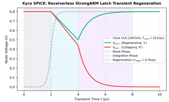
Fig. 6. Xyce SPICE transient simulation of the receiverless clocked StrongARM dynamic latch at 100 GHz. Regeneration occurs in \tau_{\text{regen}} = 0.78 ps, completing binary decision latching in under 8 ps.
