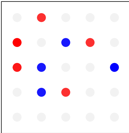
GCN Subject 1
