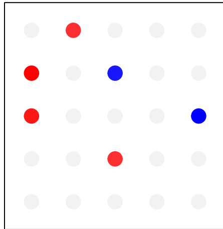
GCN Subject 3
