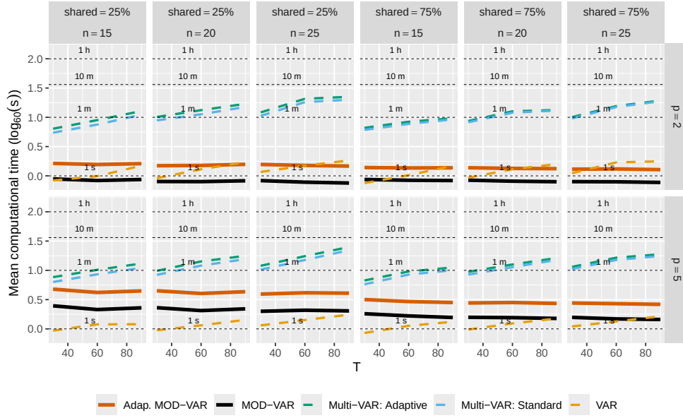
Figure S13: Visualization of the mean log-computational time for our proposed MOD-VAR and methods in the literature for data where the heterogeneity across subjects consists of only moderator-dependent components, with no subject-specific components. We explore performance for d = 10 , varying n , T , p and the proportion of shared/moderated components.
