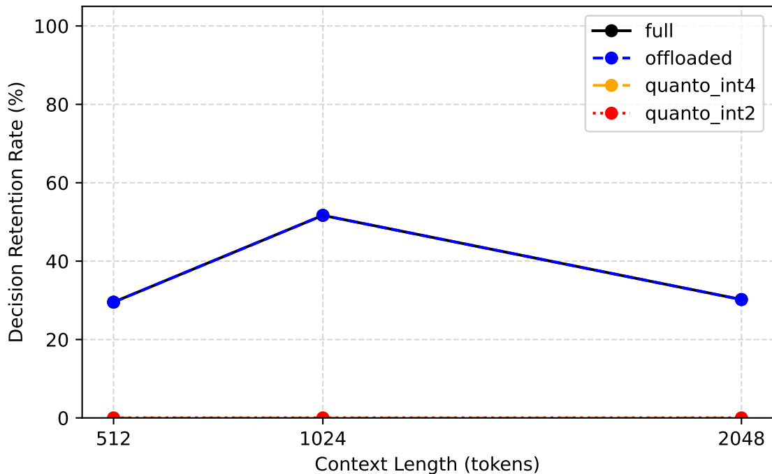
Tool Decision Retention vs. Context Length
