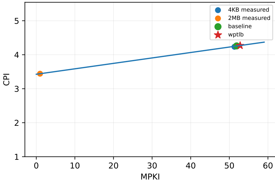
spec_cpu2017/605.mcf_s
