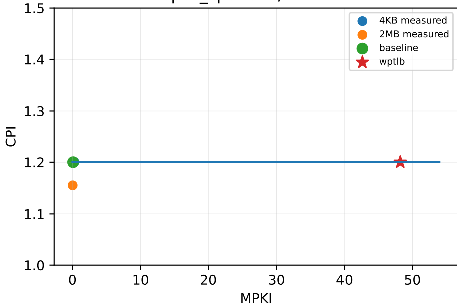
spec_cpu2006/429.mcf
