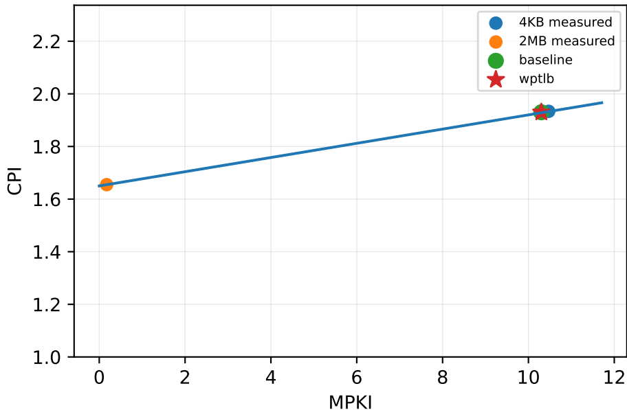
gapbs/sssp-kron-4GB
