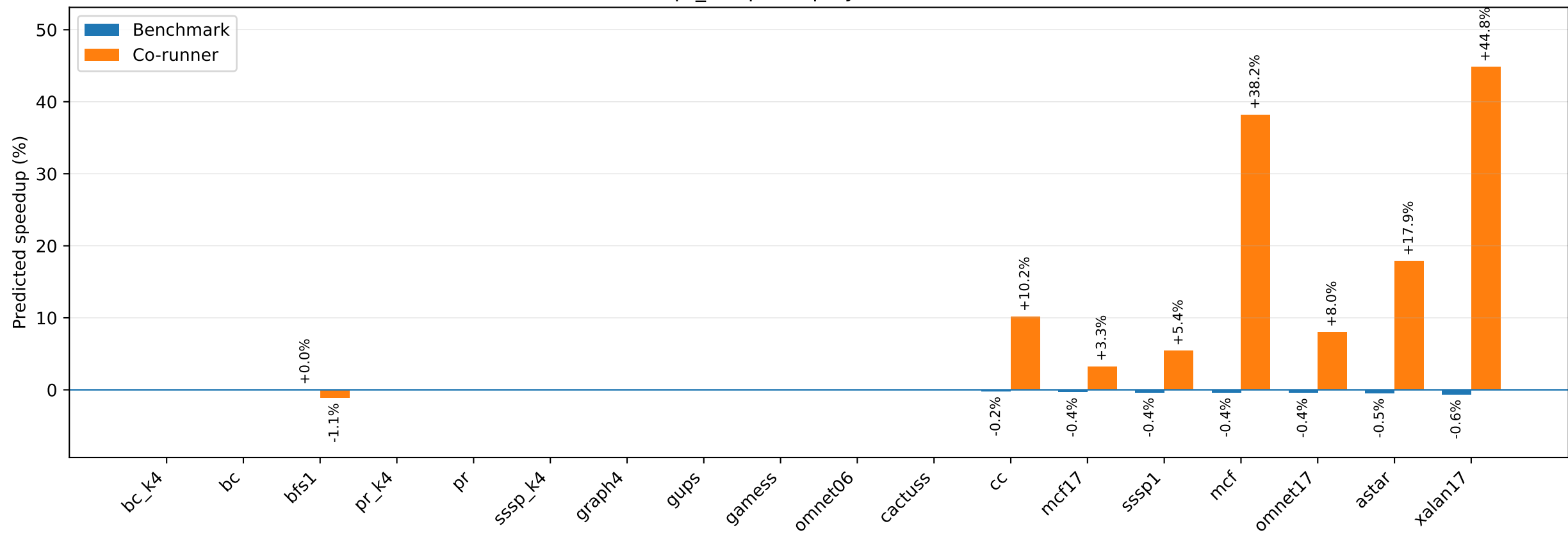
pr_k4 speedup by co-runner
