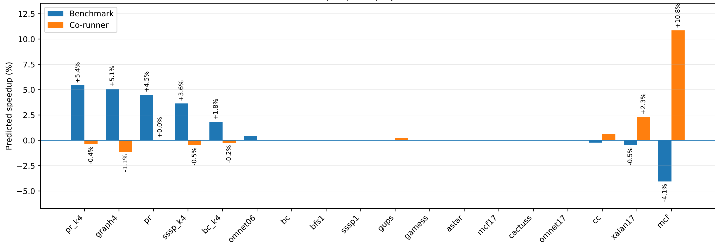
sssp1 speedup by co-runner
