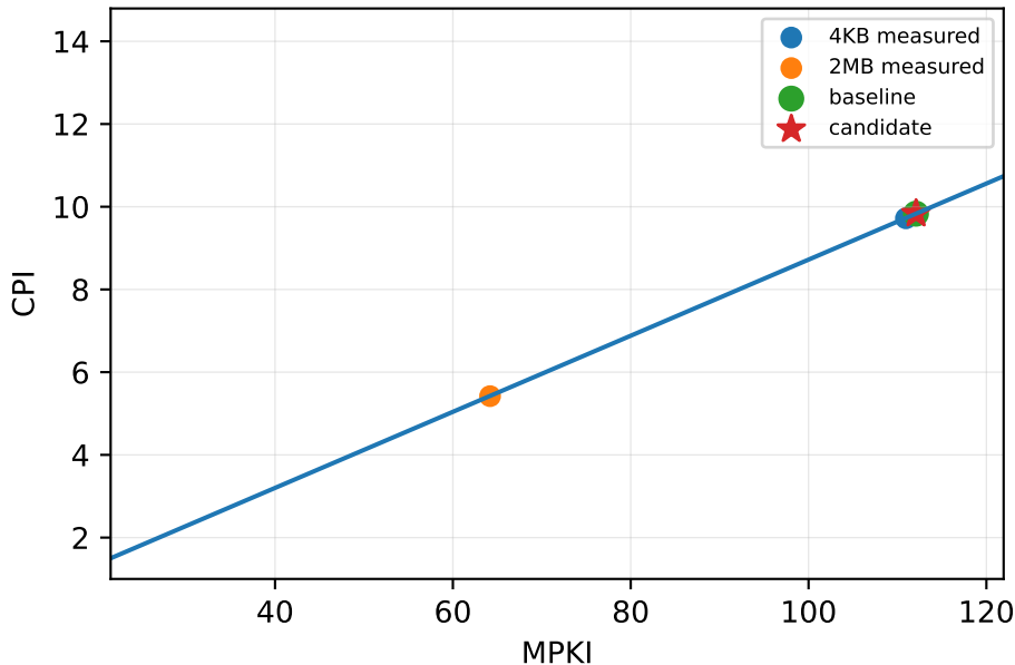
gapbs/sss-kron-4GB
