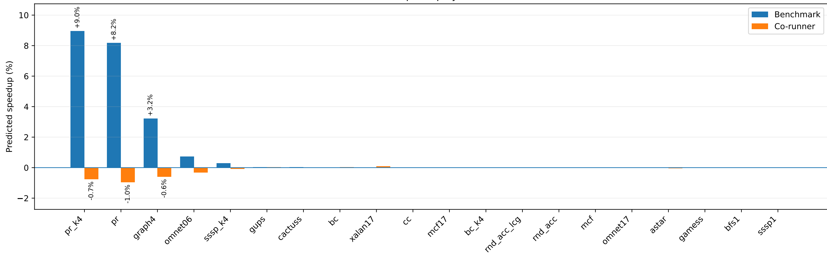
omnet17 speedup by co-runner
