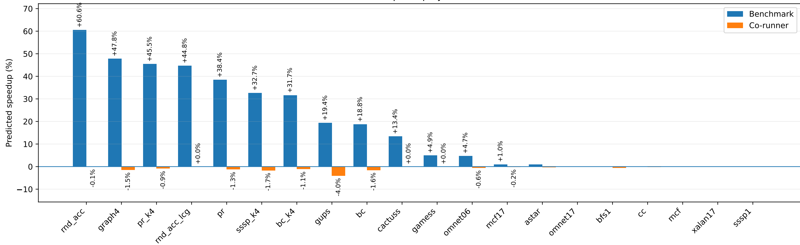
xalan17 speedup by co-runner
