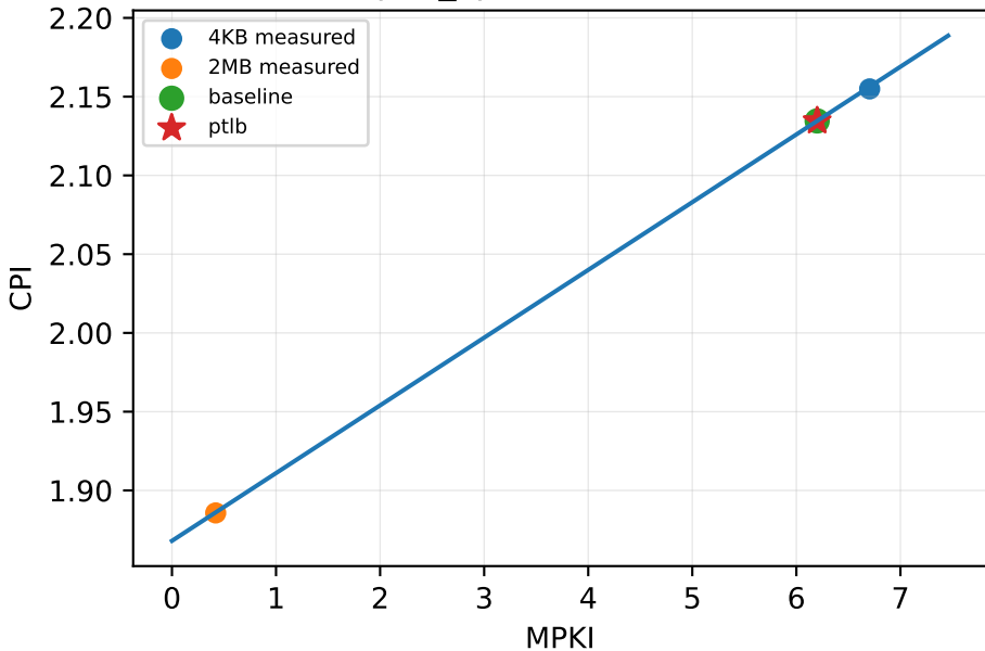
spec_cpu2006/429.mcf
