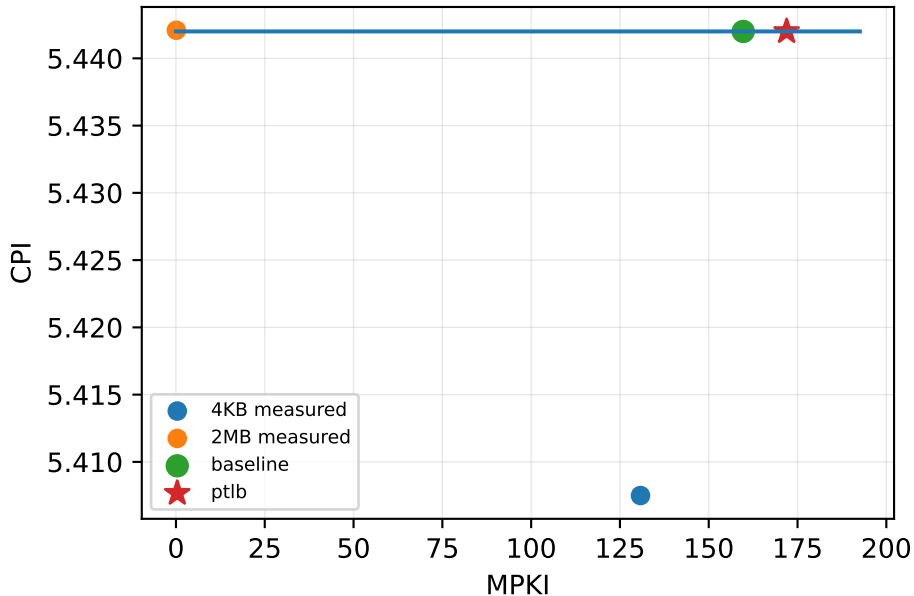
spec_cpu2006/471.omnetpp
