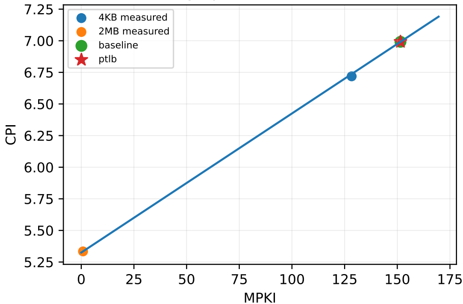
graph500-2.1/4GB
