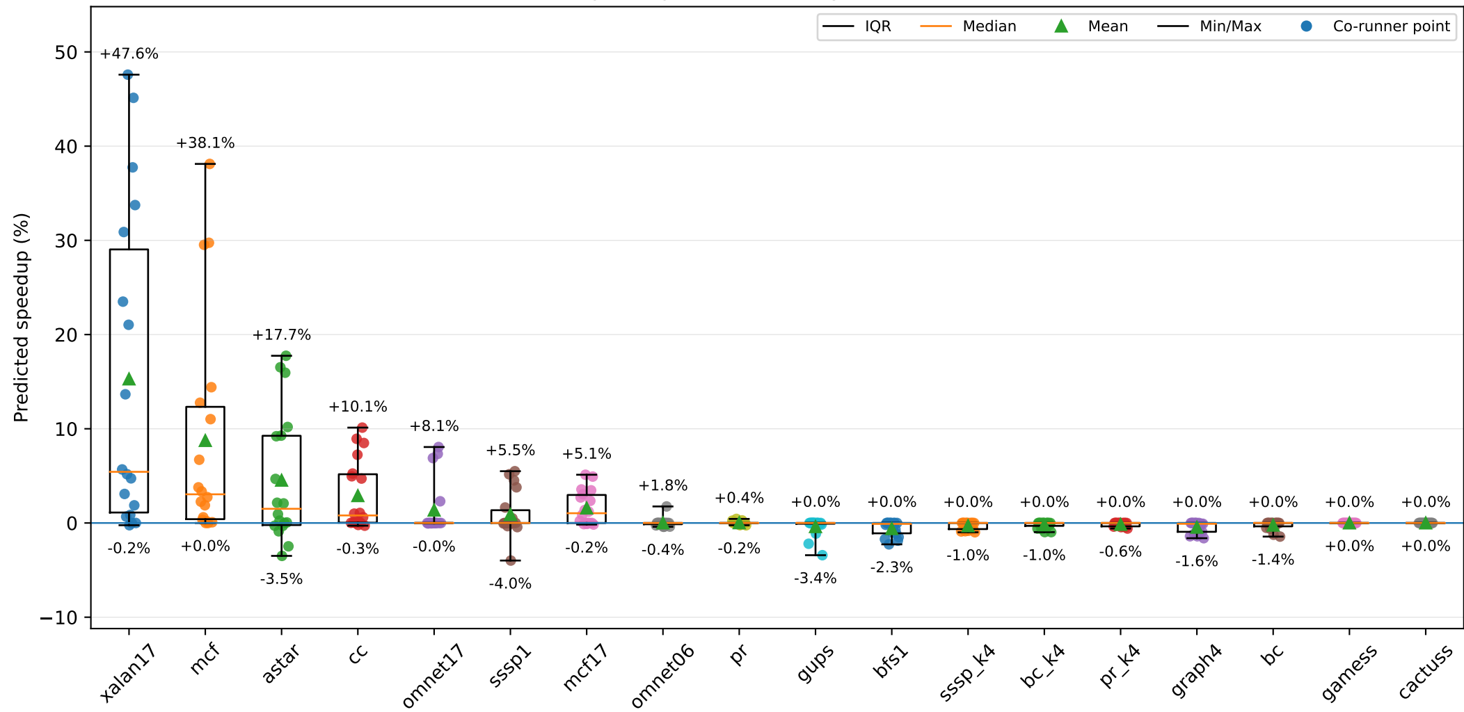
Speedup distribution by benchmark
