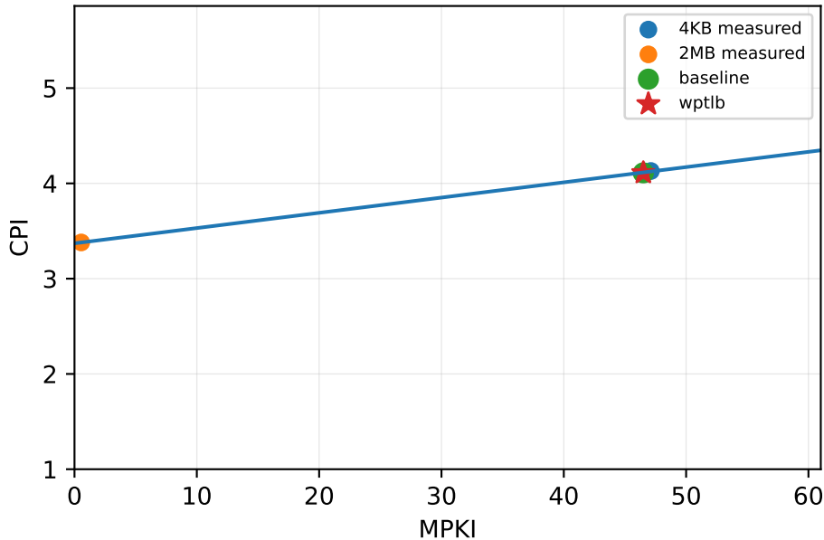
gapbs/bfs-urand-1GB
