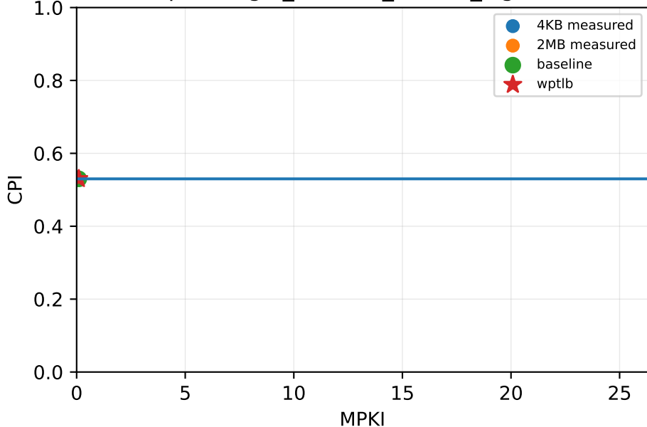
hpcc/single_random_access_lcg-4GB
