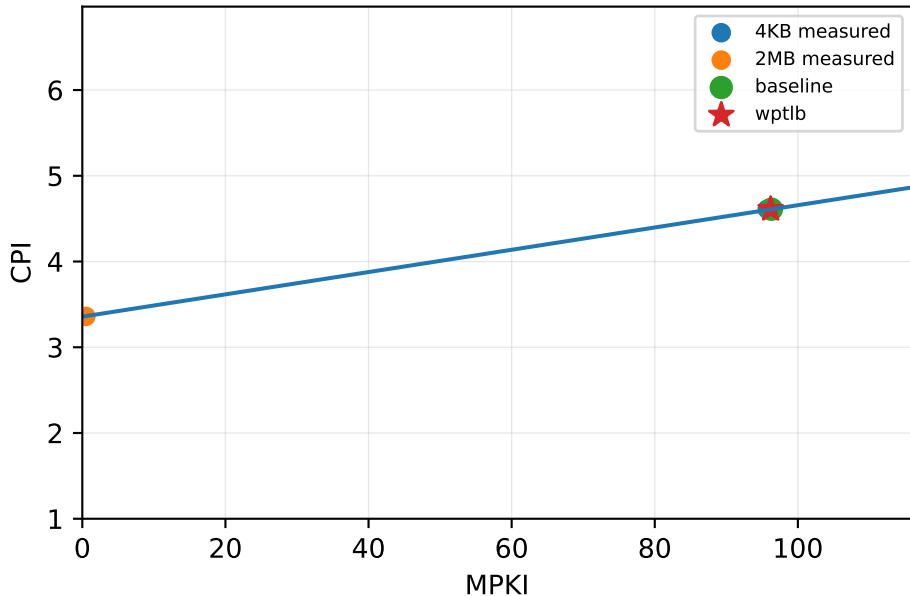
gapbs/bc-urand-4GB
