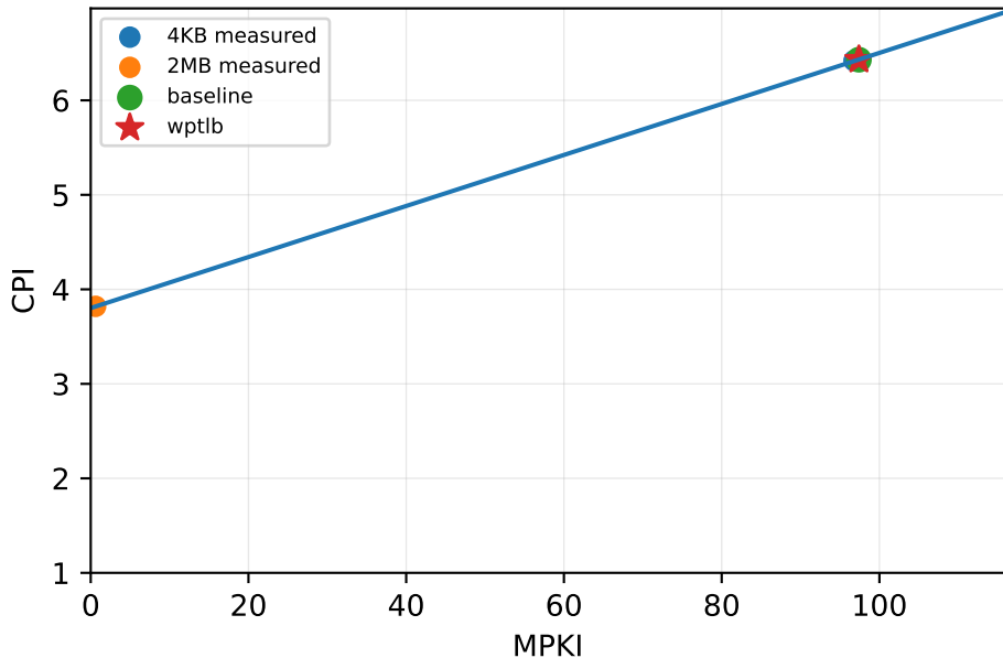
hpcc/single_random_access_lcg-4GB
