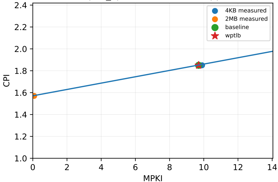
spec_cpu2006/471.omnetpp
