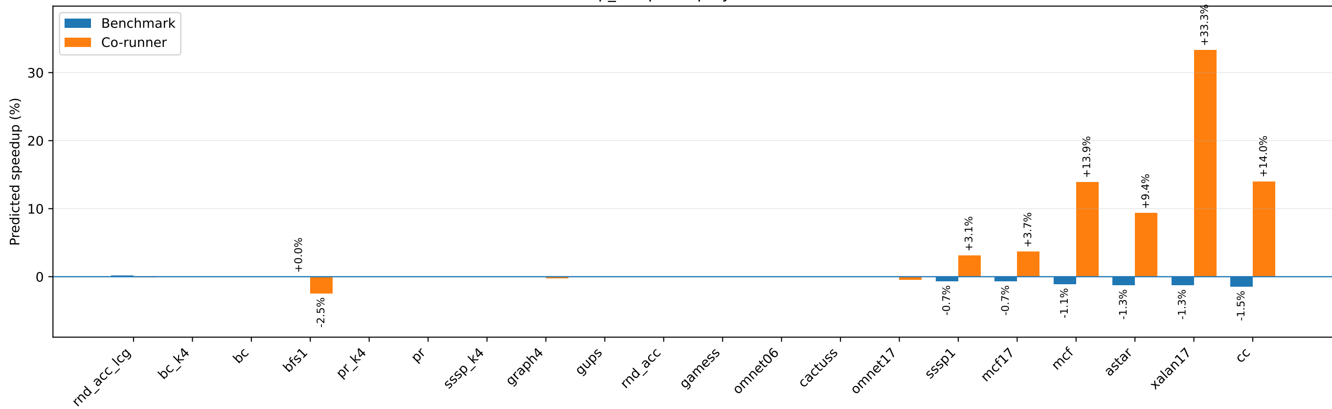
sssp_k4 speedup by co-runner
