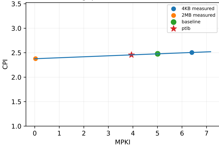
gapbs/bfs-urand-1GB
