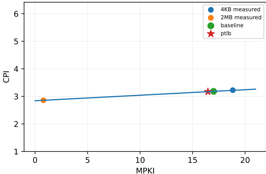
gapbs/cc-urand-4GB
