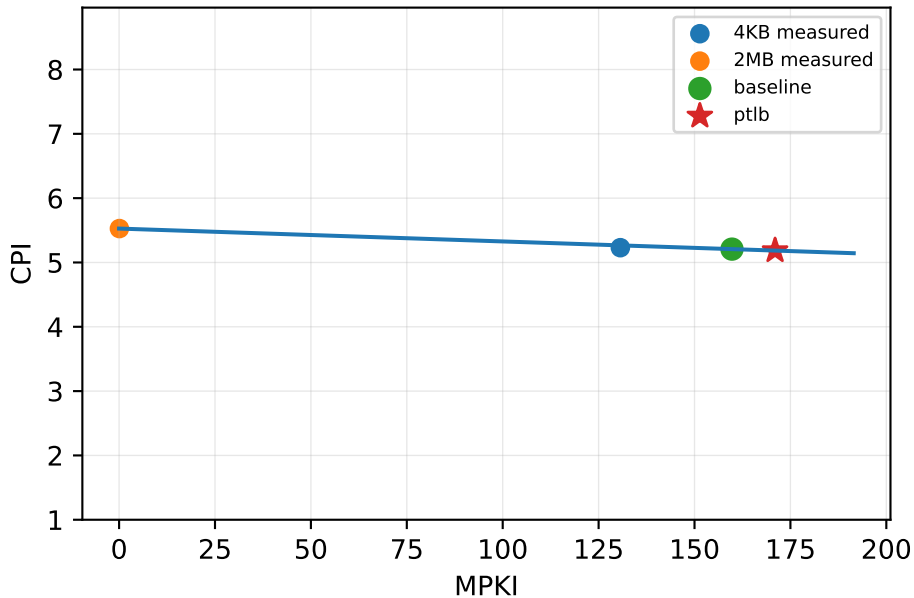
gapbs/cc-urand-4GB
