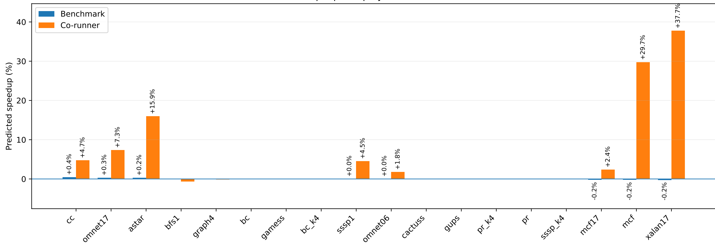
pr speedup by co-runner
