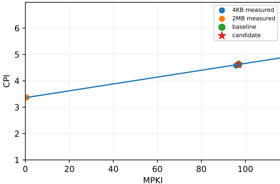
gapbs/bc-kron-4GB
