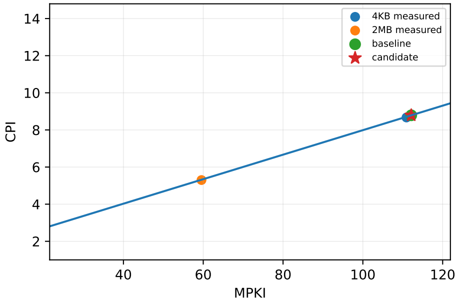
spec_cpu2017/605.mcf_s
