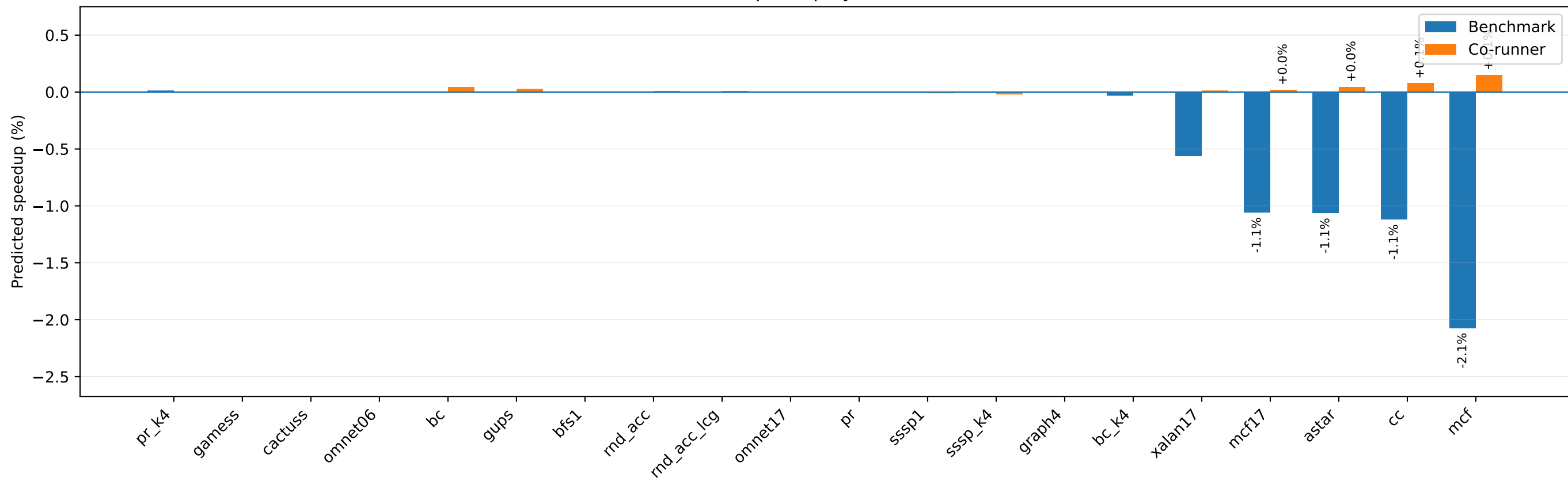
bfs1 speedup by co-runner
