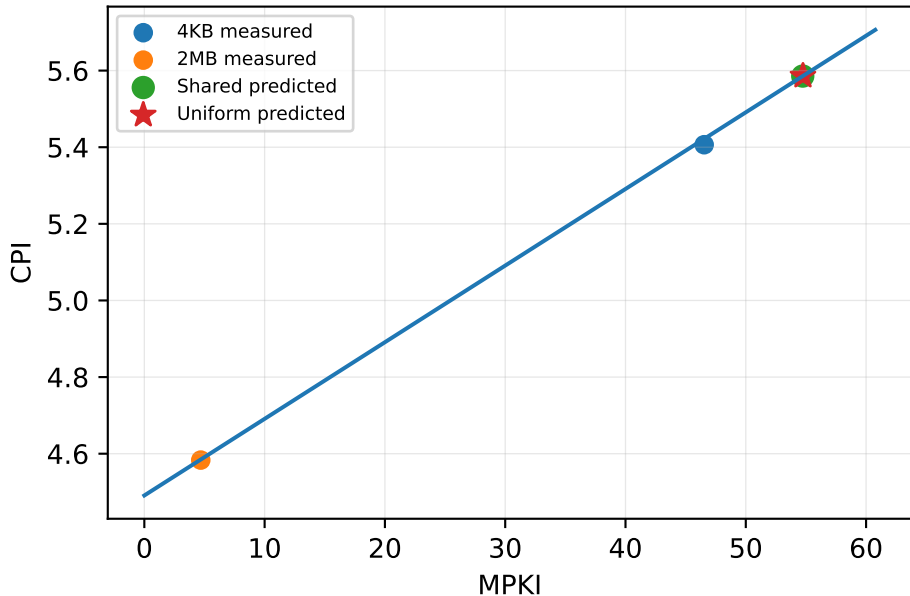
gapbs/sssp-urand-1GB
