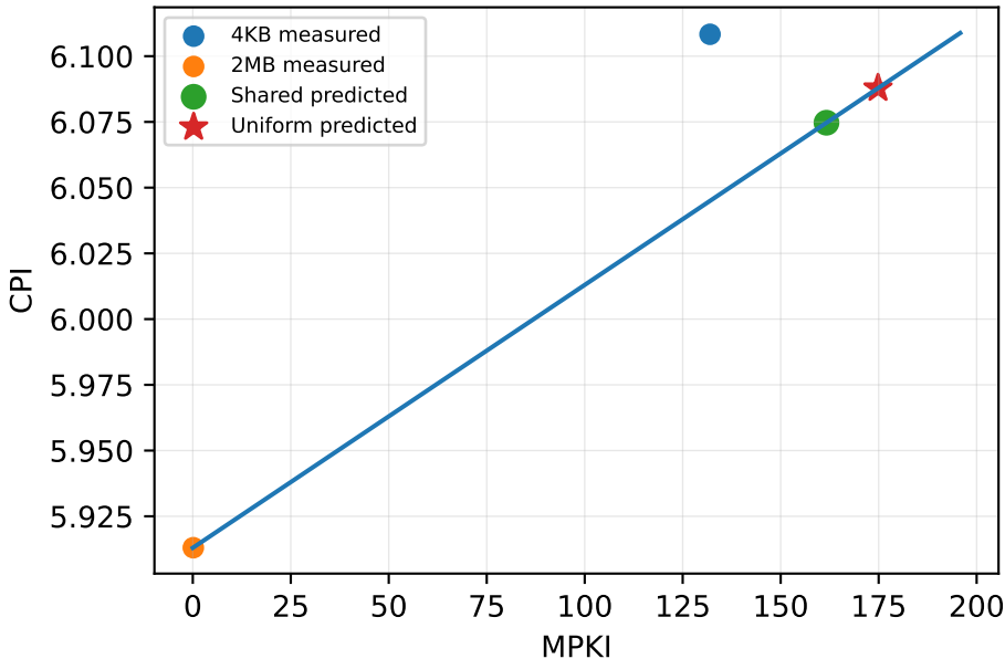
spec_cpu2006/429.mcf
