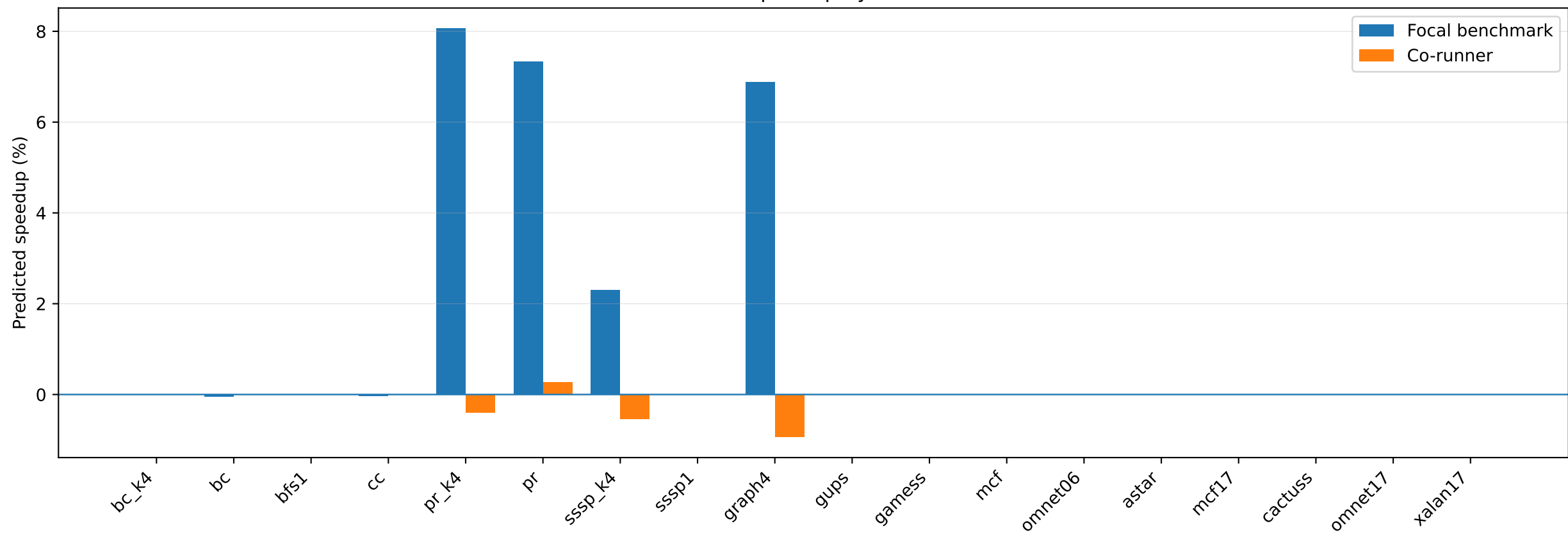
omnet17 speedup by co-runner
