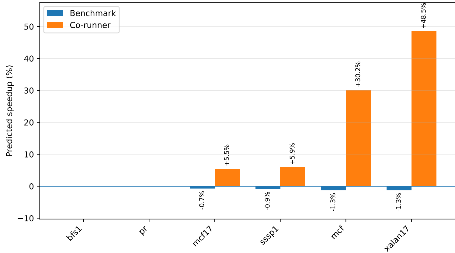
graph4 speedup by co-runner
