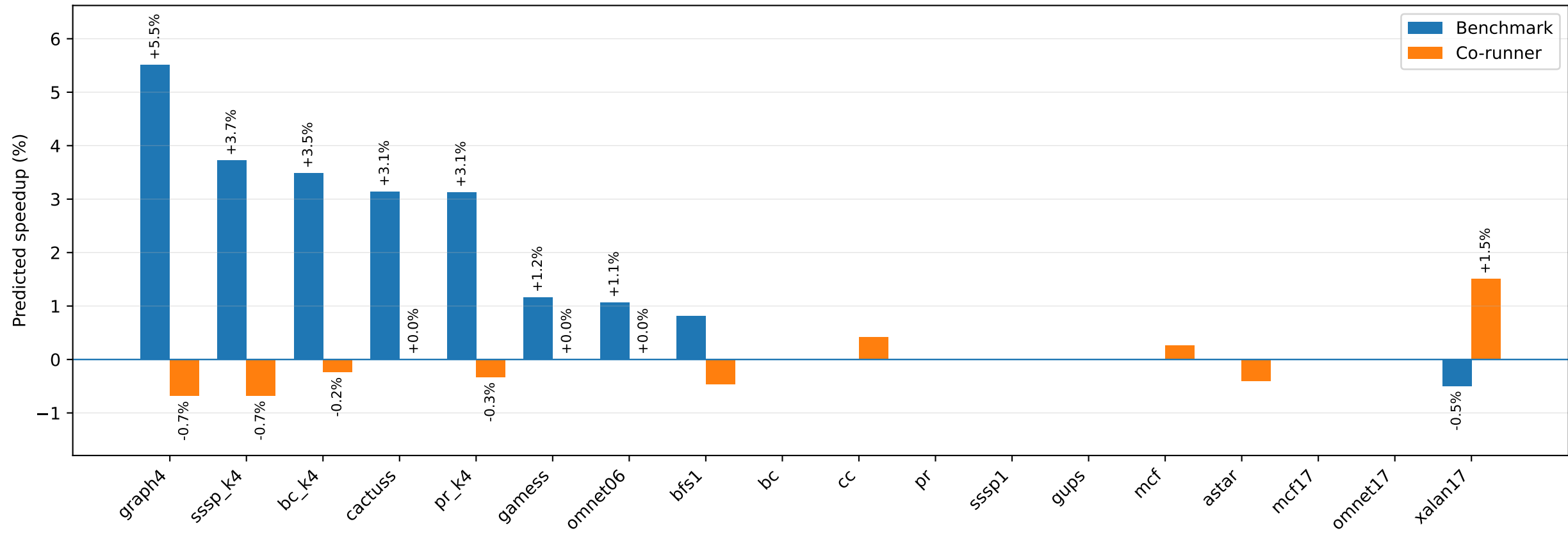
mcf17 speedup by co-runner
