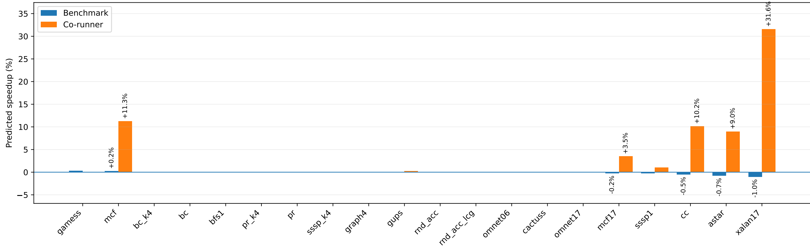
bc_k4 speedup by co-runner
