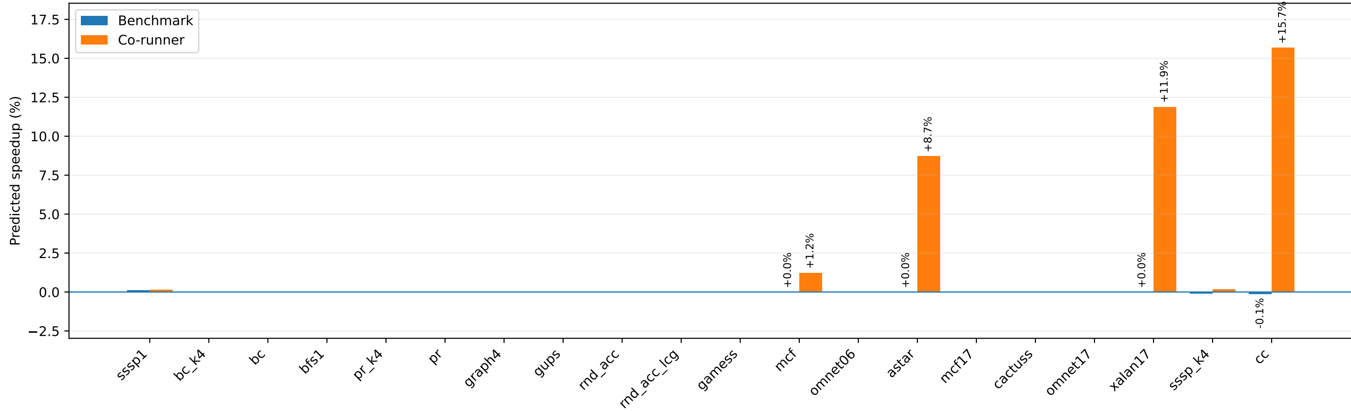
rnd_acc_lcg speedup by co-runner
