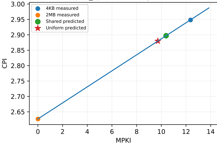
spec_cpu2006/416.gamess
