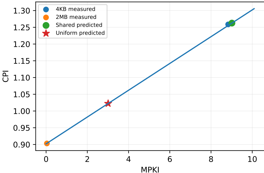
gapbs/bc-urand-4GB
