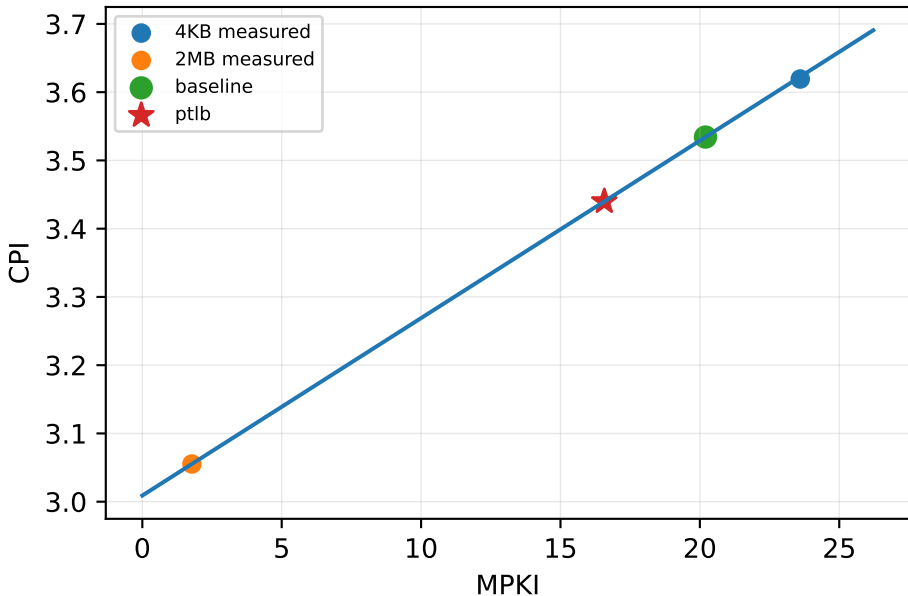
spec_cpu2006/471.omnetpp
