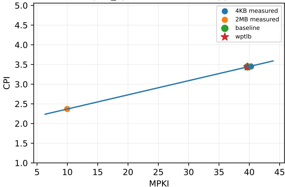
spec_cpu2006/471.omnetpp
