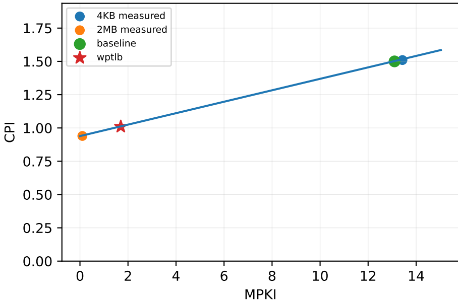
graph500-2.1/4GB
