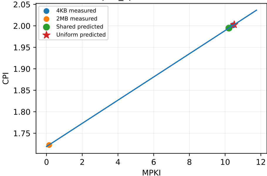
spec_cpu2006/429.mcf
