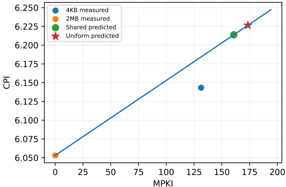
spec_cpu2017/605.mcf_s
