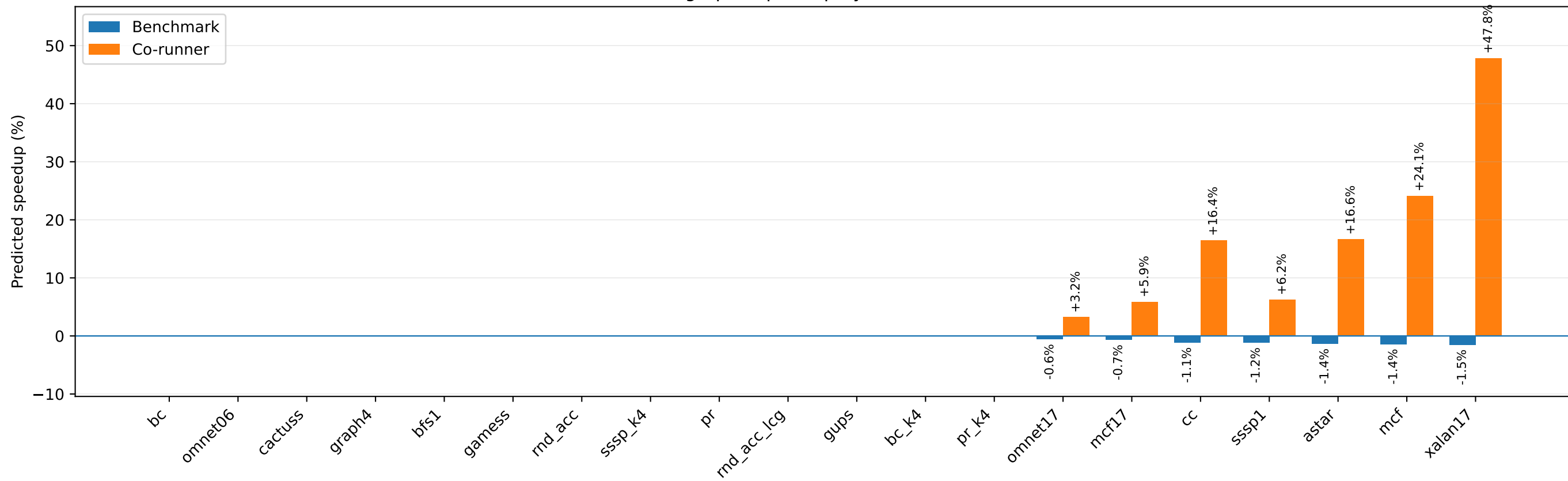
graph4 speedup by co-runner
