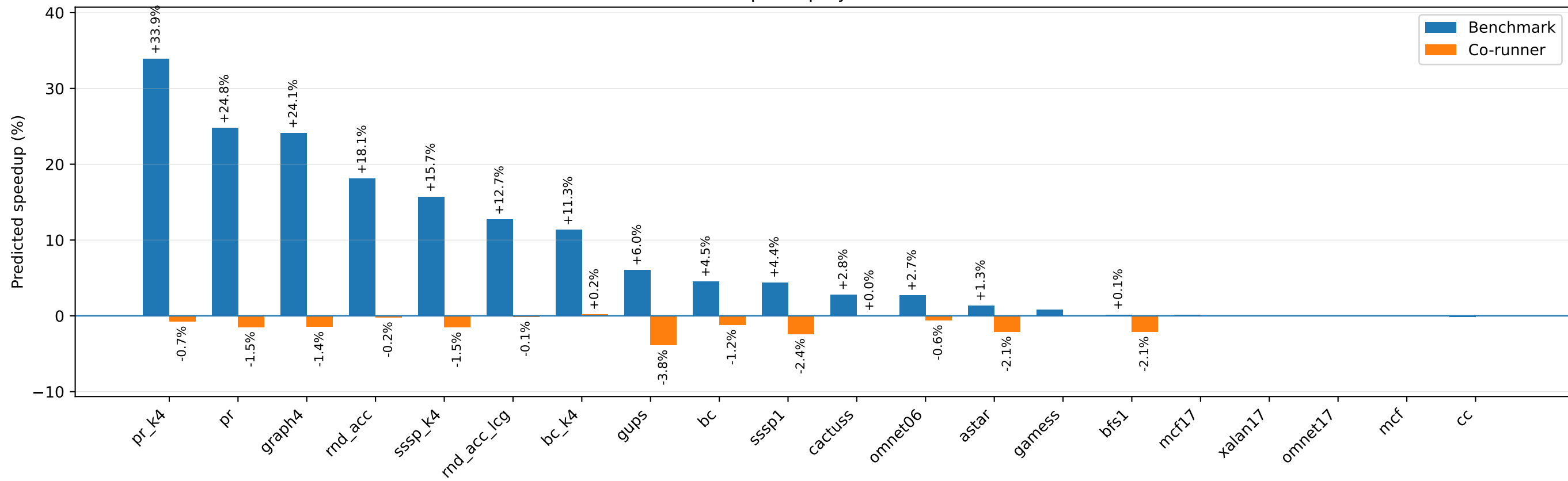
mcf speedup by co-runner
