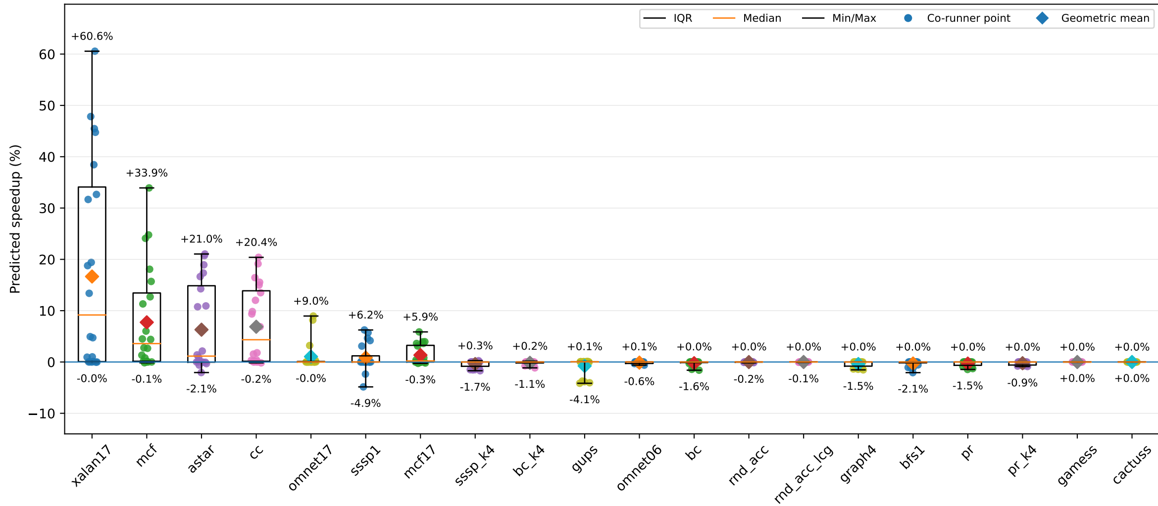
Speedup distribution by benchmark
