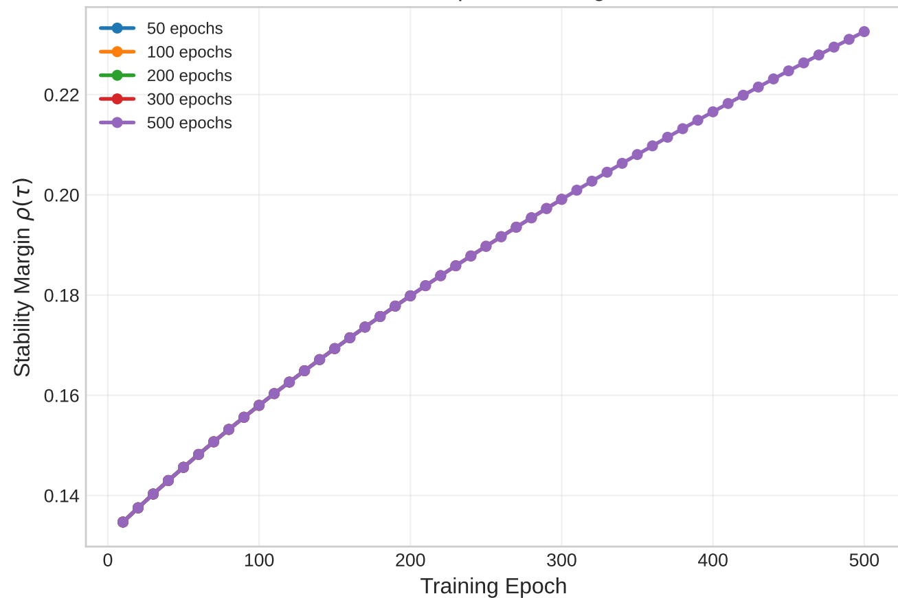
IEEE 118: Epoch Convergence
